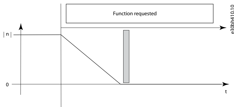
Illustration 22: SLS Monitoring Motor Speed
