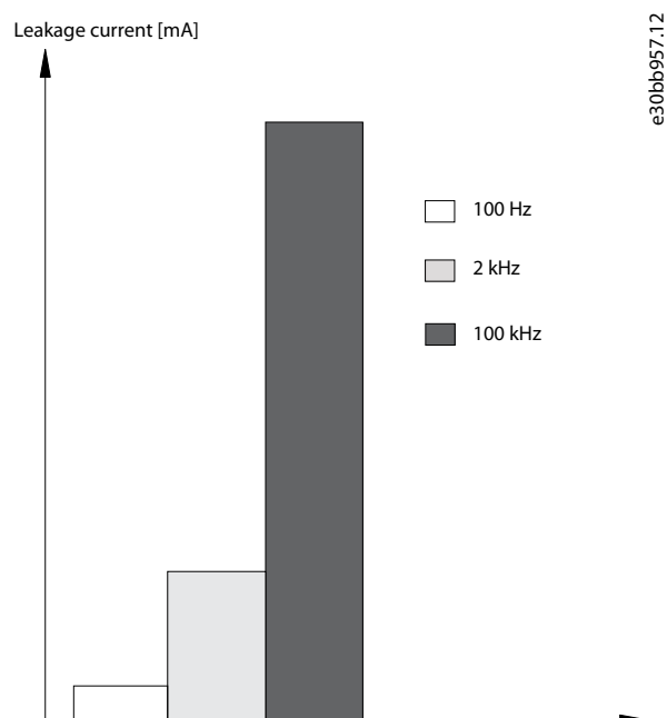
Illustration 134: Influence of Cut-off Frequency of the RCD on what is Responded to/Measured
